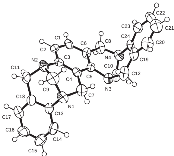
FIG. 2 ORTEP (ref. 18 ) drawing of X-ray structure of 7a
