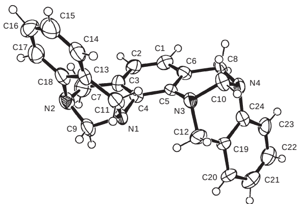
FIG. 3 ORTEP (ref. 18 ) drawing of X-ray structure of 7b
